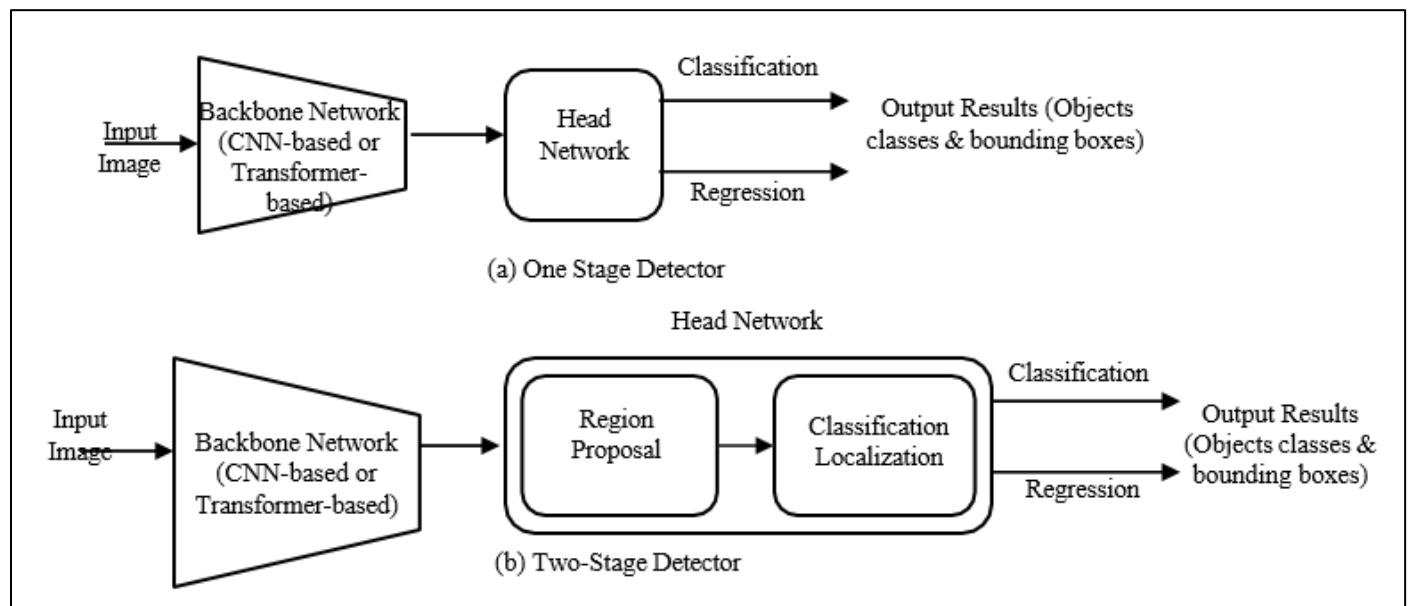
Fig 1 System One Stage and Two Stage Detector Methodology
