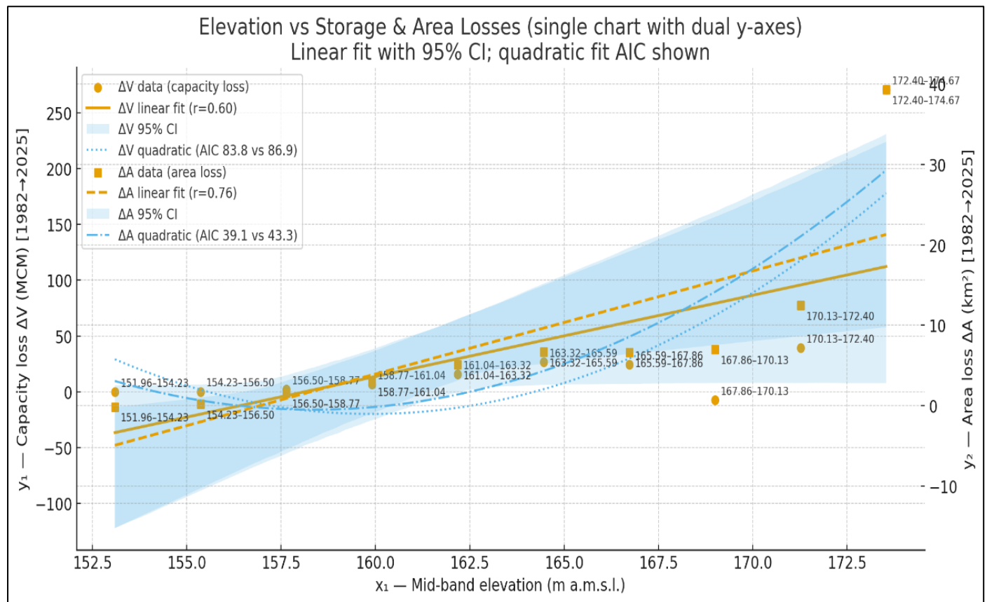
Fig 7 Elevation-Dependent Capacity ( \Delta V ) and Area ( \Delta A ) Losses, Kiri Dam (1982–2025):
