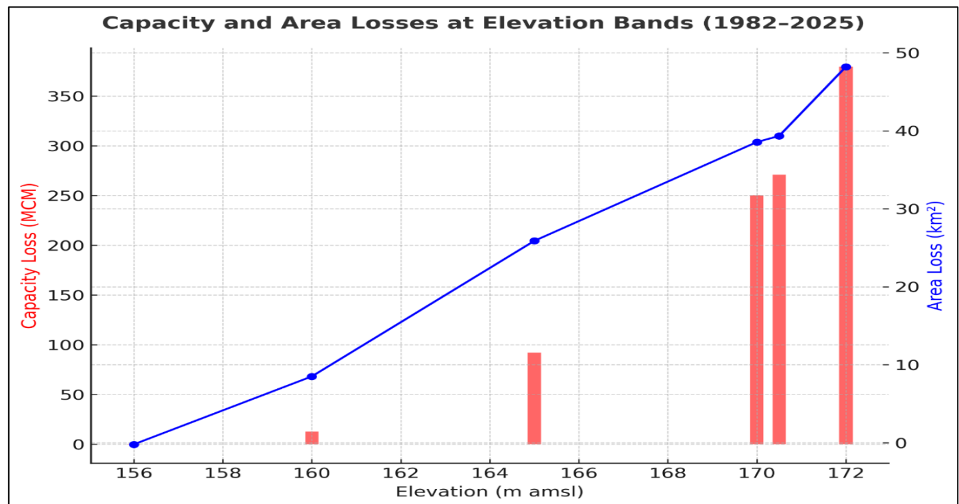
Fig 4 Capacity and Area Losses at Elevation Bands (1982–2025)
