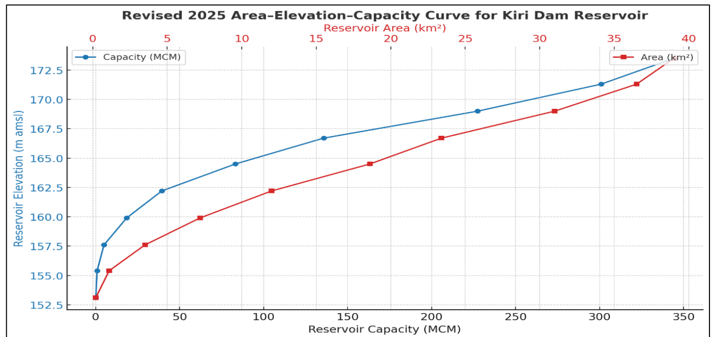
Fig 3 Revised 2025 Area–Elevation–Capacity Curve for Kiri Dam Reservoir
