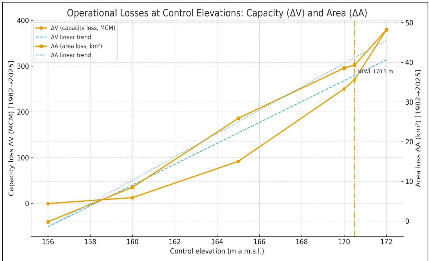
Fig 6 Capacity Loss ( \Delta V , MCM) and Area Loss ( \Delta A , \text{km}^2 ) Versus Control Elevations; NTWL at 170.5 m Indicated.
