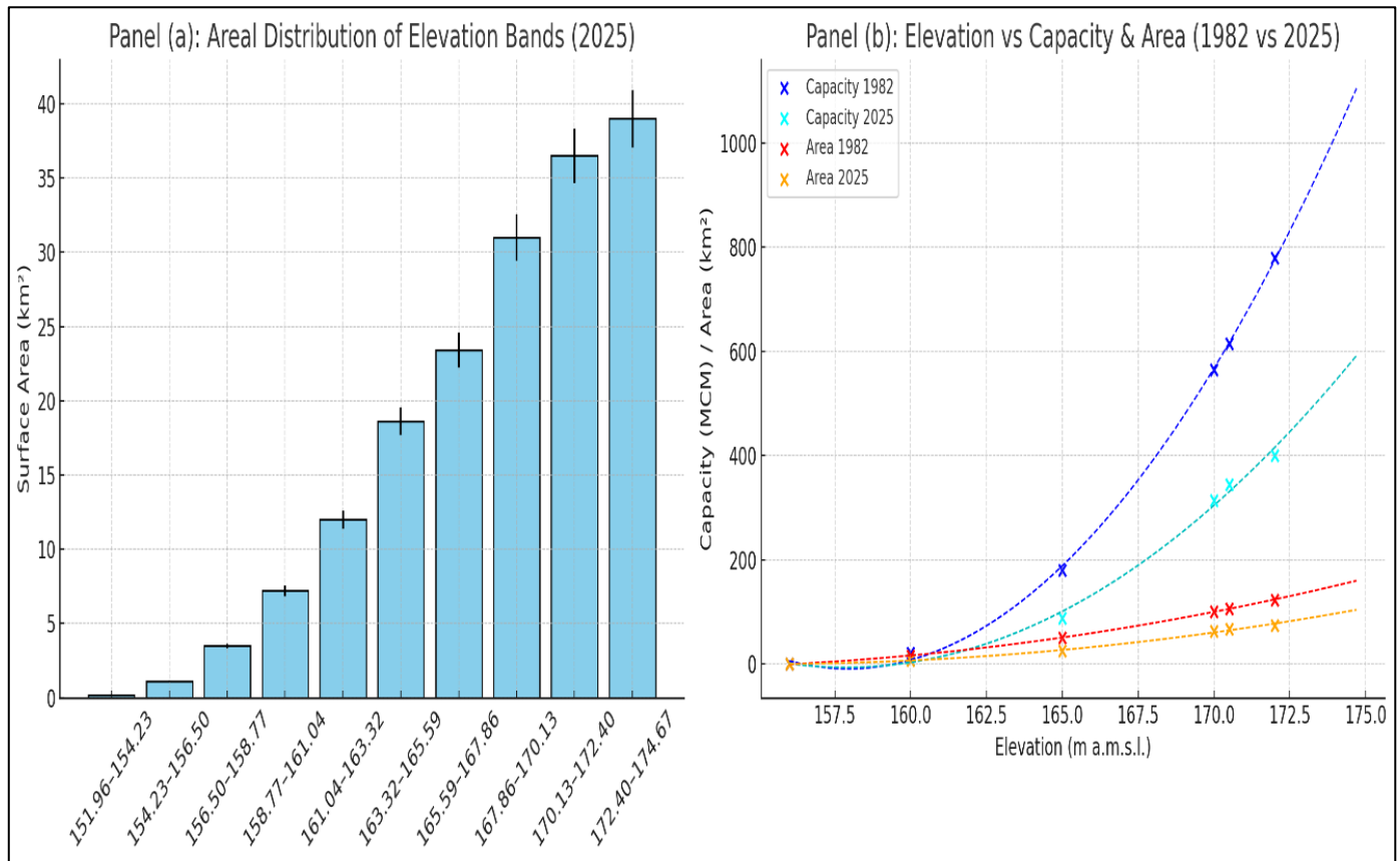
Fig 5 Areal Distribution and Statistical Correlation of Elevation Bands (2025):
