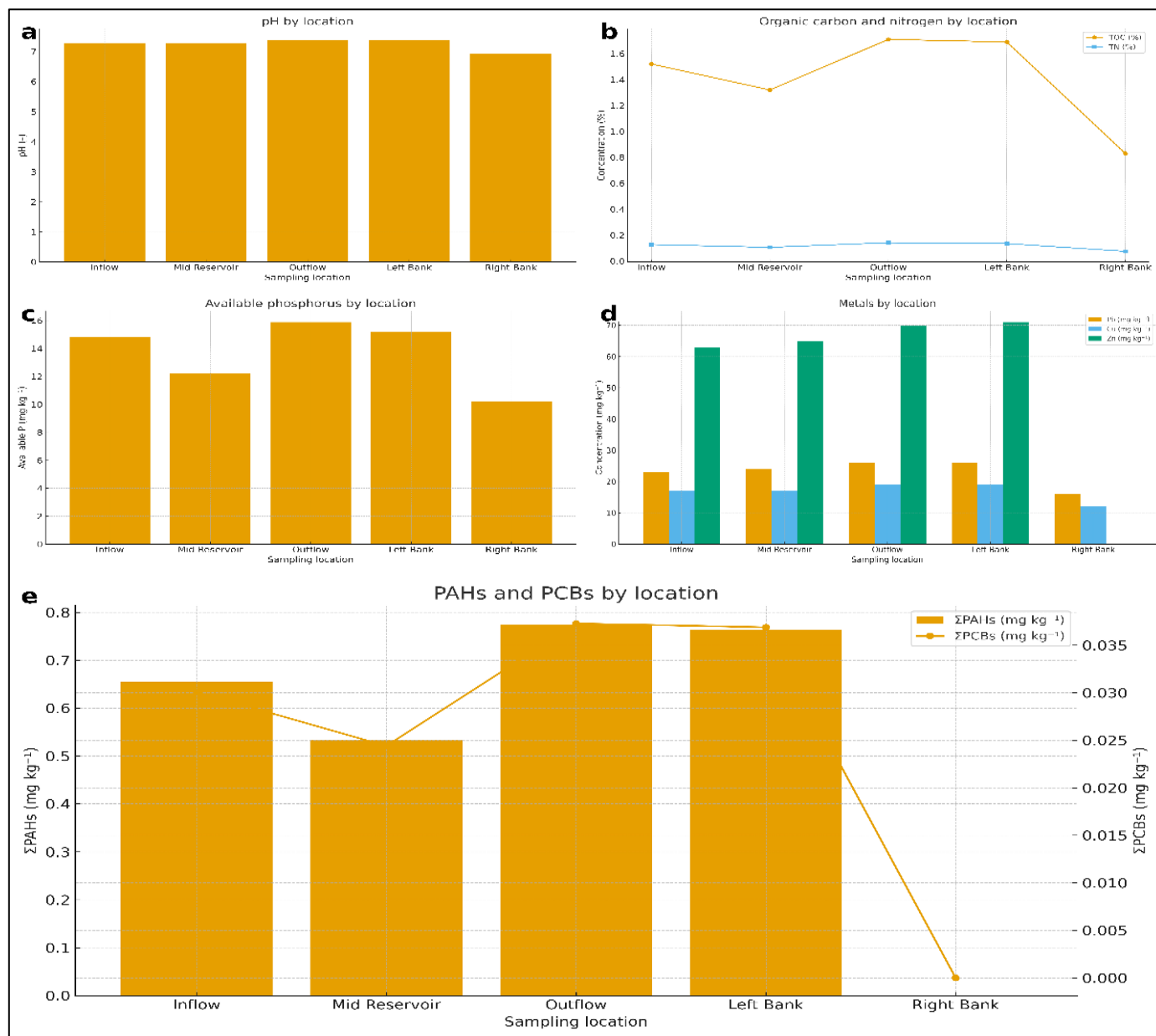
Fig 9 A-E. Spatial Variation of Sediment Geochemistry by Location in Kiri Dam (2025).
