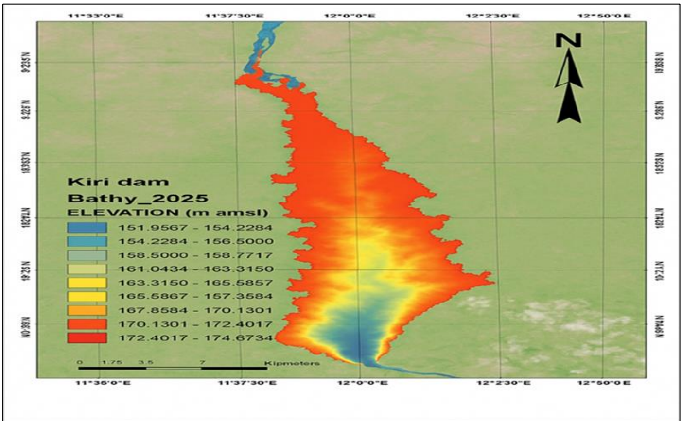
Fig 1 Bathymetric Survey Map of Kiri Reservoir Bed Topography (2025)
