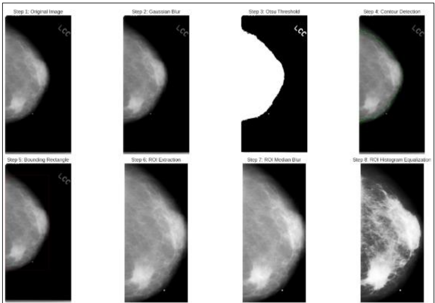
Fig 2 Data Preprocessing
