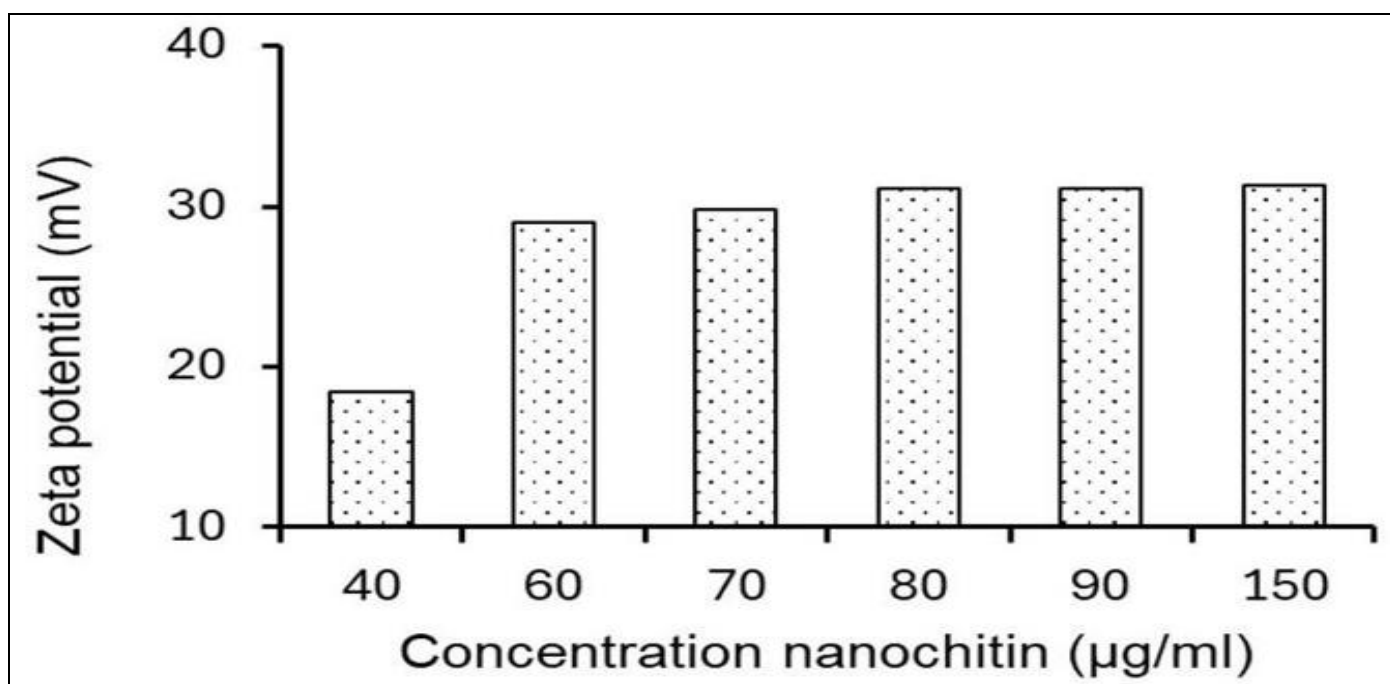
Fig 2 Zeta Potential of Nanochitin Solutions at Different Concentrations
